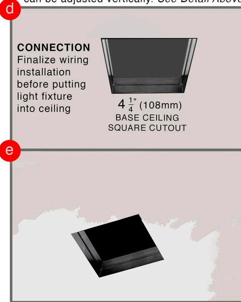
Step D - Install ceiling and cutout square opening to fit around housing throat.
