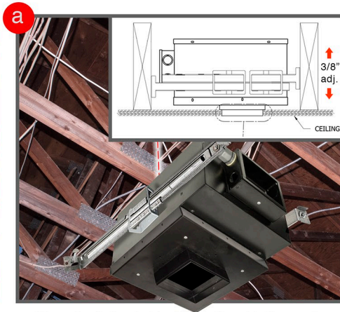
Step A - Adjustable Mounting Rails anchor housing to ceiling joists with screws. Housing can be adjusted vertically. See Detail Above.
