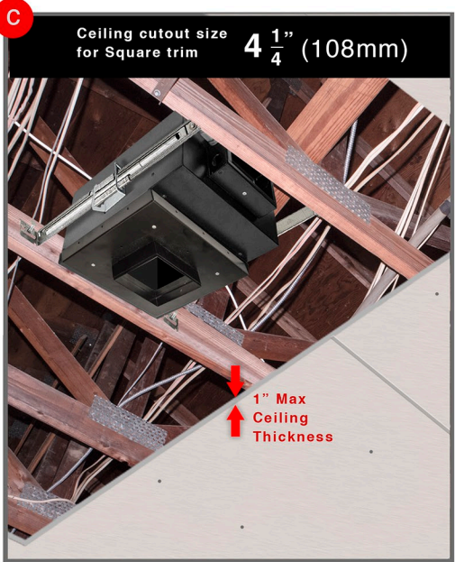
Step C - Finish base ceiling installation.
