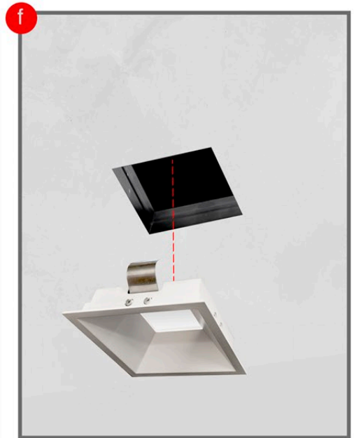
Step F - After paint has dried out, clip in flanged trim to finalize install.
