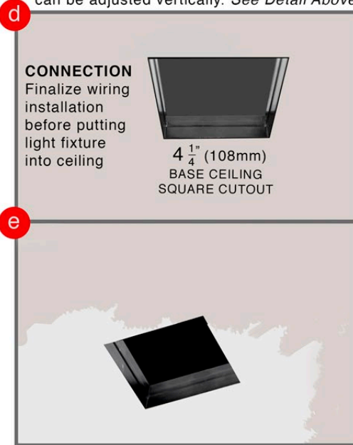
Step D - Install ceiling and cutout square opening to fit around housing throat. Step E - Paint ceiling after GWB has been cut to fit around housing throat.
