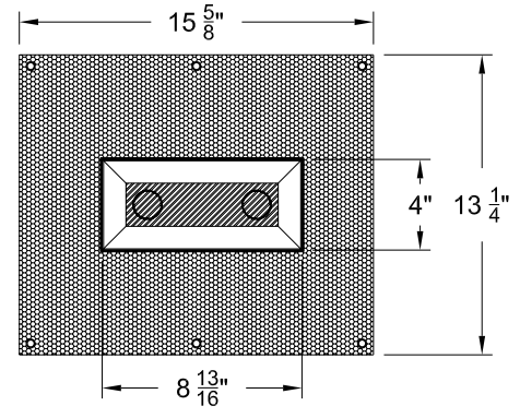
REFLECTED PLAN VIEW
